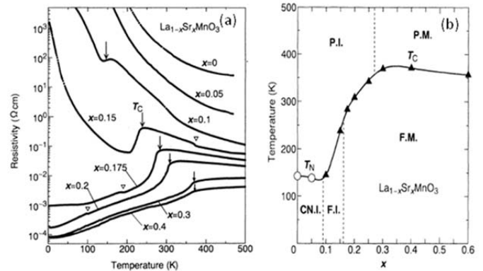
Fig. 3. (a) Resistivity of \text{La}_{1-x}\text{Sr}_x\text{MnO}_3 as a function of temperature. The arrows indicate critical temperatures for magnetic transitions. (b) The phase diagram of the \text{La}_{1-x}\text{Sr}_x\text{MnO}_3 system. The abbreviations F, P, CN, M, and I stand for ferromagnetic, paramagnetic, spin-canted antiferromagnetic, metallic and insulating, respectively [2].
