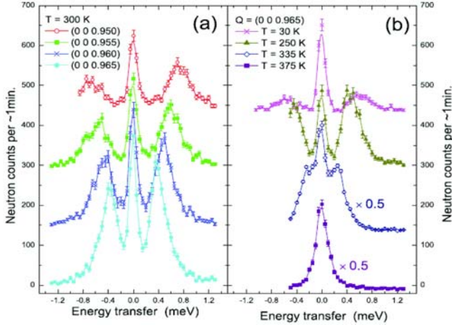
Fig. 9. Constant-Q scans revealing spin wave excitations for \text{La}_{0.7}\text{Sr}_{0.3}\text{MnO}_3 (a) at T = 300 K, for several wave vectors, and (b) Q = (0\ 0\ 0.965) , for several temperatures [5].
