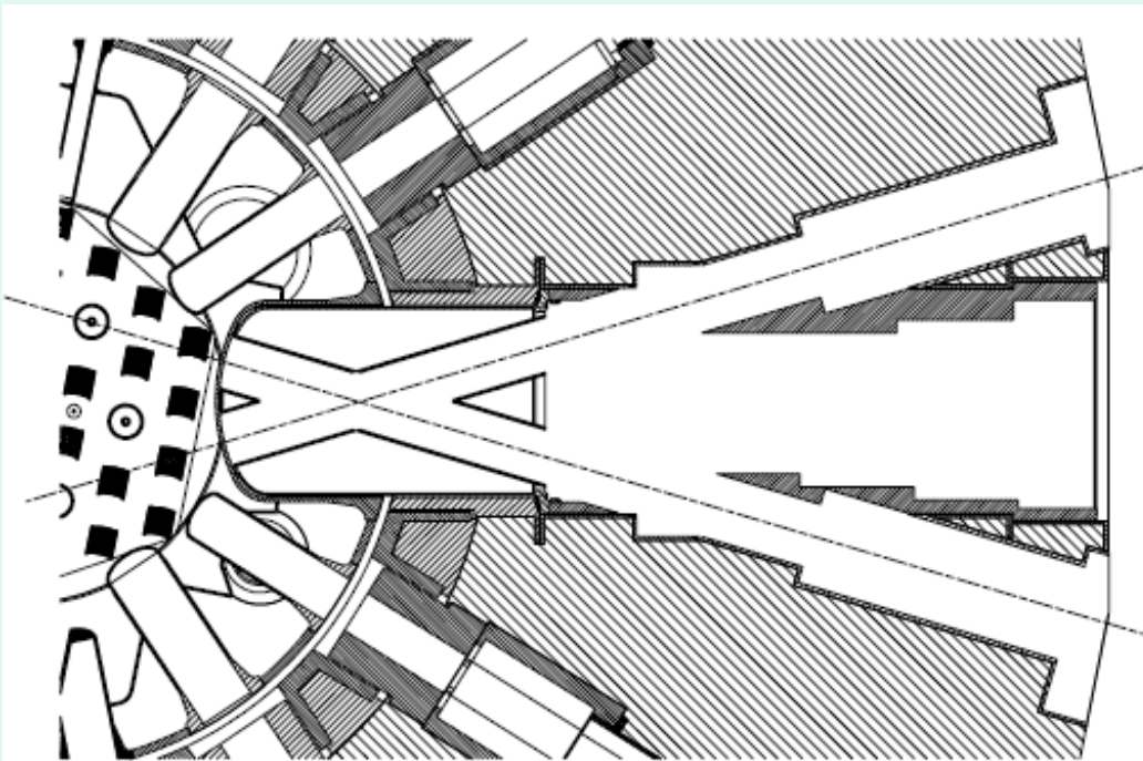
Figure 2.2. Original layout of the cold neutron port.
