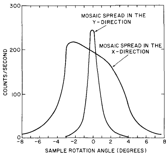
Fig. 11. The two histograms presented here are the "rocking curves" for an assembly of thin Thermica crystals separated by wedges of aluminum as described in the appendix. There were 15 such sub-units having one 0.01'' piece of mica sandwiched between 0.005'' pieces of aluminum. The resulting curves indicate a larger mosaic width in x than in y as desired.
