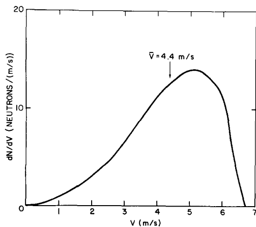
Fig. 8. The velocity distribution of neutrons in the bottle is plotted. The average velocity is 4.4 m/s for v_{\text{max}} = 7 m/s. The parameters in table 2 were used as input to the Monte Carlo program, dN/dv is the number of neutrons per unit velocity increment.
