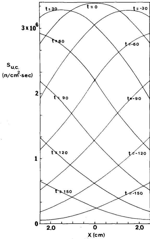
Fig. 5. This figure shows the ultra-cold neutron source intensity S_{u.c.} at various times t as a function of position x across the crystal face. The parameters of table 2 were used as input data.
