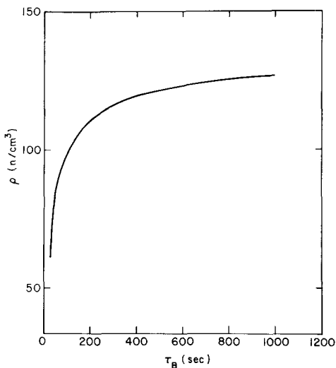
Fig. 9. The expected asymptotic storage density of neutrons in the bottle after many pulses is plotted versus the bottle storage time, \tau_B . The parameters input for the Monte Carlo program were set using table 2. The crystal reflectivity was taken to be 100%.
