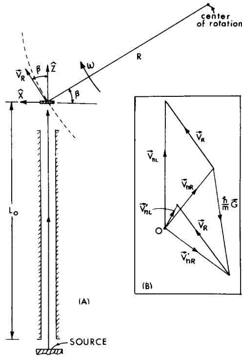
Fig. 2. This figure defines the symbols used in the text to describe the Doppler-shifter as viewed in the laboratory (A) and as viewed in velocity space (B). The velocity vector \mathbf{v}_R of the moving crystal makes an angle \beta with the beam center line ( \mathbf{z} ) when the center of the crystal passes the beam center. The nominal Bragg angle \theta_B is related to \beta by \theta_B = \frac{1}{2}\pi - \beta .
