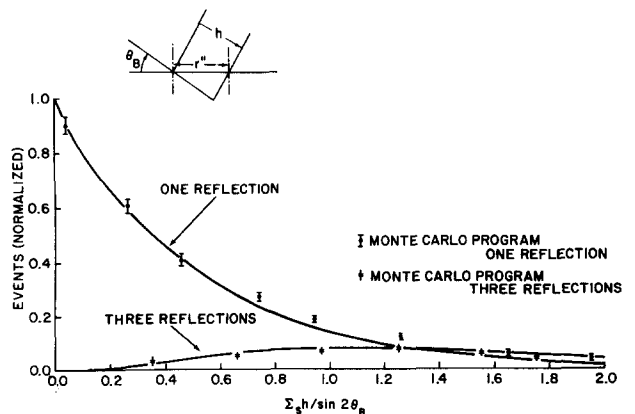
Fig. 7. This figure shows a comparison between the Monte Carlo simulation of multiple reflections within the crystal and the analytic calculation taken from ref. 37. The slight differences observed are due to the finite crystal size taken in the Monte Carlo simulation whereas the calculation assumed a semi-infinite crystal.
