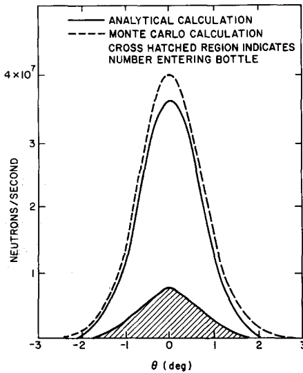
Fig. 6. The total ultra-cold neutron production rate, which is the integration of the curves of fig. 5 over the crystal area, is plotted here as a function of the rotor angle \theta = \omega t (solid curve). The y -dimension of the crystal was taken to be 5 cm, while the x -dimension was 2 cm. Also shown are the results for the Monte Carlo simulation (dashed curve). The cross-hatched region is the number of neutrons arriving in the bottle. Parameter values were set using table 2. The crystal reflectivity \gamma_0 was taken to be 100%.
