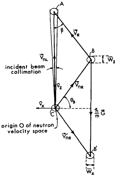
Fig. 3. This diagram shows the velocity space volumes effective in the Doppler-shifting process, and how the neutron distributions as viewed in the laboratory (L) and in the moving (R) frames are related. The dimensions W_z = 2.35 W'_z and W_x = 2.35 W'_x are given by eqs. (10) and (9) respectively. The third dimension W_y = 2.35 W'_y of volumes B' and C is given by eq. (11).
