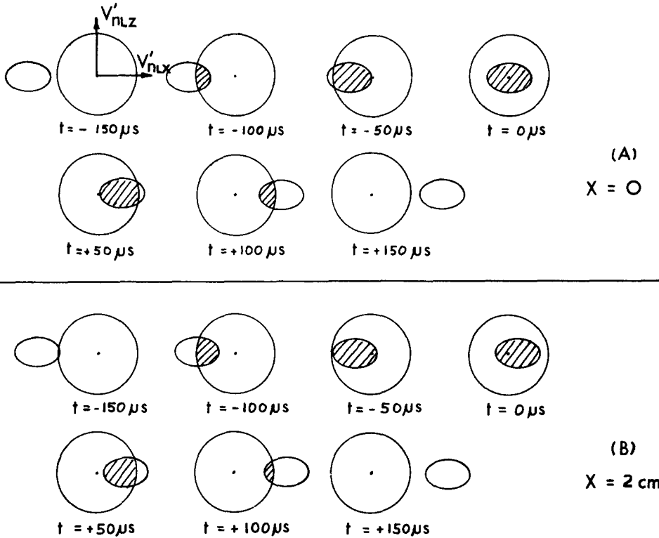
Fig. 4. This figure shows the overlap (shaded region) of the Doppler shifted neutrons with a sphere of radius v_{\max} in the v'_{xL} - v'_{zL} plane. The top part (A) of the figure is for the point x = 0, y = 0 on the crystal face. The bottom part (B) of the figure is for a point x = 2 cm, y = 0 . The machine parameters used to construct these figures are given in table 2.
