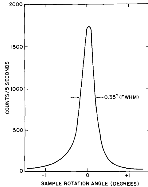
Fig. 10. This histogram is the "rocking curve" for a piece of Thermica described in the appendix. The measurements were made at the National Bureau of Standards reactor in a 2.24 \text{ \AA} neutron beam. The sample dimensions were 1'' \times 1'' and 0.01'' in thickness.
