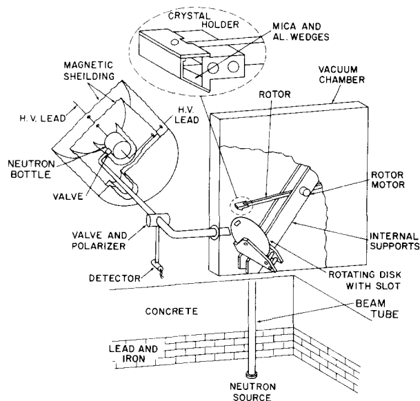
Fig. 1. An overall schematic diagram of the apparatus to be used to search for the neutron EDM at the pulsed sources at Argonne National Laboratory. The Doppler-shifter (rotor) is currently being tested at the ZING-P' source. It is 2.4 m in diameter and turns at 30 Hz.
