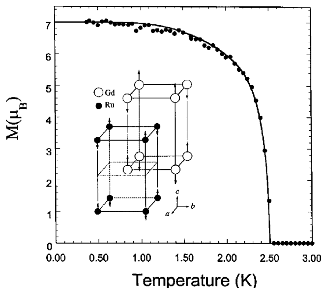
FIG. 5. Gd sublattice magnetization vs T . The Néel temperature is 2.50 K. The inset shows the magnetic structures for the Ru and Gd.
