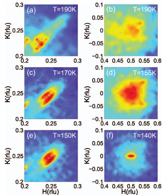
FIG. 2. (Color) Panels (a), (c), (e) show mesh scans around the AF Bragg peaks (0.25,0.25,0) at T = 190 , 170, and 150 K. Panels (b), (d), (f) show mesh scans around (0.5,0,0) at T = 190 , 155, and 140 K.
