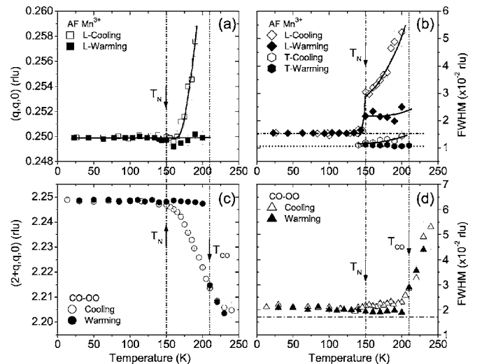
FIG. 4. Temperature dependence of (a) propagation wave vector and (b) FWHM for Mn^{3+} AF ordering. The corresponding T dependence of (c) propagation wave vector and (d) FWHM for CO-OO. "L" refers to the [1\ 1\ 0] direction and reflects the interchain coupling. "T" refers to the [-1\ 1\ 0] direction and is associated with the intrachain coupling. Dashed lines indicate the instrumental resolution.
