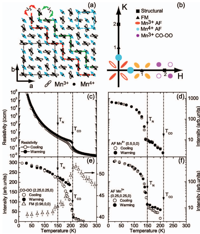
FIG. 1. (Color) Panel (a) shows schematic diagram of the CE-type structure in the nearly half doped perovskite manganites in the cubic setting. The zigzag chains formed by alternating Mn 3+ and Mn 4+ spins are coupled antiferromagnetically, the coupling within the chain is ferromagnetic. The short-dashed line denotes the periodicity of the Mn 3+ orbital and magnetic unit cell, long-dashed line shows the Mn 4+ magnetic unit cell. Panel (b) depicts the corresponding superlattice peaks in the reciprocal space (solid symbols). Open symbols indicate superlattice peaks that are forbidden in a single-domain crystal but are observed because of twinning. Bottom: Temperature dependence of (c) resistivity; (d) AF peak intensity from (0.5,0,0); (e) CO-OO peak intensity from (2.25,0.25,0) and FM short-range fluctuations from (0.96,0,0); and (f) AF peak intensity from (0.25,0.25,0). In panels (c)–(f) open and solid symbols represent cooling and warming, respectively.
