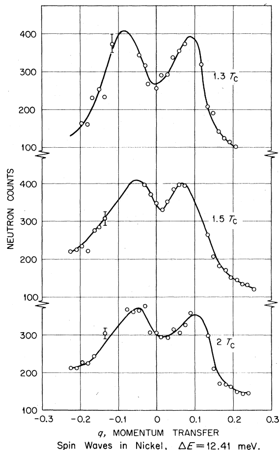
FIG. 7. Magnetic scattering at \pm q for 12.41 meV covering temperatures up to 2T_C .
