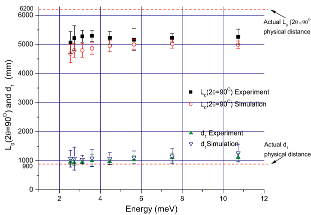
Figure 7. Energy dependence of the focusing parameters L_0(2\theta = 90^\circ) and d_1 versus energy. The dashed lines show the actual physical distances. The deviations indicate optimization that accommodates aberrations between the simplified focusing calculation that is used to determine the monochromator setting and the more complicated physical reality of the instrument that compensates for aberrations. Nominally, L_0(2\theta = 90^\circ) is the reference position distance from source to monochromator and d_1 is the perpendicular distance from reactor beamline to the center of the MBT drum. To extract the optimal value of L_0(2\theta = 90^\circ) and d_1 the corresponding scans were fitted to a third-order polynomial. The error bars represent one standard deviation.
