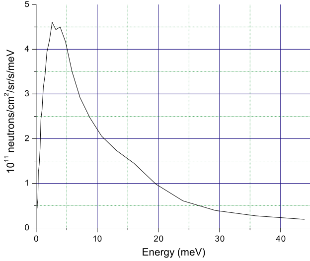
Figure 4. Cold source brightness. The cold source intensity was calculated using Monte Carlo N -particle transport code (MCNP) [8].
