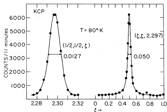
FIG. 3. Observed scattering at the CDW satellite position (0.5, 0.5, 2.297) . The scan on the left-hand side is "through" the 2k_F plane, i.e., along the c -axis direction. The width is limited by the instrumental resolution, and the position shows that the CDW is incommensurate with the tetragonal lattice. The scan on the right-hand side measures the interchain correlations. \zeta = 0.5 is the zone boundary of the tetragonal lattice in the [110] direction. Note the difference in abscissa scale of the two plots of this figure.
