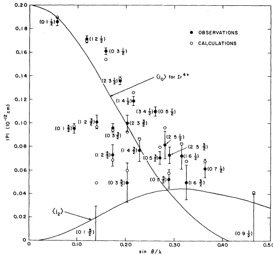
FIG. 1. Measured form factor with p = (0.27 \times 10^{-12} \text{ cm}/\mu_B) \mu f(\vec{K}) in absolute units. The data not only differ sharply from spherical symmetry, but they also do not show cubic symmetry.
