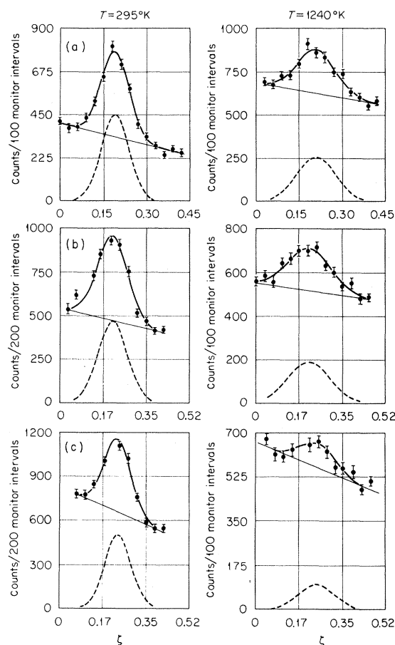
FIG. 4. Comparison of spin waves with energies of (a) 70.3 meV, (b) 95.1 meV, and (c) 103.4 meV, at room temperature and 1240 °K for \vec{Q} = (1 + \xi, 1 + \xi, 0) . The spin waves at high temperatures are reduced in intensity and broadened, but are still easily observable.
