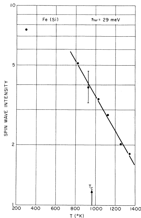
FIG. 5. Temperature dependence of the spin-wave intensity for E = 29 \text{ meV} . The intensity decreases about four times faster than can be accounted for in terms of the Debye-Waller factor.
