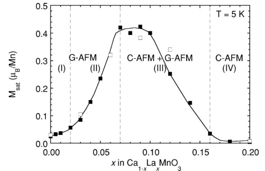
FIG. 3. Magnetic saturation moments M_{sat} determined from M vs H curves at 5 K for the samples used in the present study (open squares) and in the study by Neumeier and Cohn (Ref. 25) (solid squares) as a function of x . Regions (I)–(IV) discussed by Neumeier and Cohn are labeled and defined by dashed lines.
