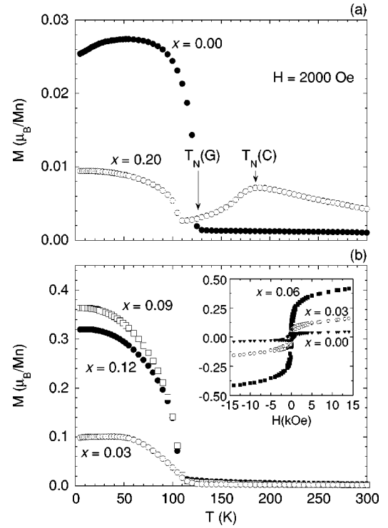
FIG. 2. (a) Magnetization M vs T measured at H=2000 Oe for x=0.00 and 0.20 samples. T_N(C) and T_N(G) are indicated. (b) A similar plot (note the change in scale) for x=0.03 , 0.09 and 0.12 samples, with an inset showing M vs H for x=0.00 , 0.03 and 0.06 . For the M vs H loops, lines were drawn through the low and high field regions of the data, and the intersection taken as the saturation moment M_{sat} at 5 K used in Fig. 3.
