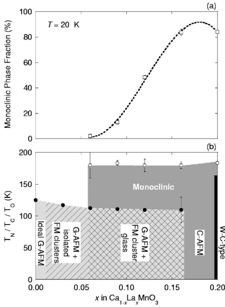
FIG. 6. (a) Refined monoclinic phase fraction at 20 K as a function of x . (b) Ground state phase diagram of \text{Ca}_{1-x}\text{La}_x\text{MnO}_3 , 0.0 \leq x \leq 0.2 , mapped onto the crystallographic and magnetic phase transitions determined from NPD data. Closed circles represent the coincident magnetic transitions T_N (G-AFM) and T_C , and open circles represent the coincident magnetic transition T_N (C-AFM) and structural transition T_O . Monoclinic (as opposed to orthorhombic) regions are dark gray. Isolated FM clusters and a FM cluster glass (to be discussed in Part II) (Ref. 16) are indicated by diagonal black lines and black diagonal cross-hatching, respectively. The WC-type phase is black. Note that at the high- x end of the G-AFM regime, the stability of the C-AFM state is very high, and therefore very little G-AFM is actually observed (a); the same is true for the W-C-type at x=0.20 , and the converse is true at the low- x end of the C-AFM regime.
