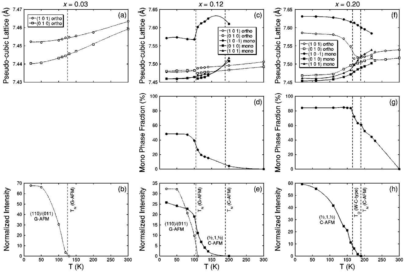
FIG. 4. (a), (c), and (f) T dependence of pseudocubic lattice parameters along (101), (101)^{\perp} , and (010) for (a) x=0.03 , (c) x=0.12 , and (f) x=0.20 , from Rietveld refinement of NPD data. Note in (c) and (f) the elongation of the monoclinic unit cell along the (101)^{\perp} direction of e_g electron polarization at T_N (C-AFM), and in (f) the elongation in the remaining orthorhombic phase of (100) and (001) due to the formation of a (twinned) Wigner-crystal type phase, in contrast to the isotropic monotonic contraction of the G-AFM orthorhombic cell in (a). (d) and (g) T dependence of the phase fraction of symmetry-lowered monoclinic ( P2_1/m ) phase associated with the C-AFM magnetic phase, from the same Rietveld-refinement of NPD data. (b), (e), and (h) T dependence of the integrated intensities of the characteristic G-AFM (110)/(011) (open circles) and C-AFM (\frac{1}{2}, \frac{1}{2}, \frac{1}{2}) (filled circles) magnetic peaks from NPD data, normalized to the intensity of the strong nuclear (220)/(022) peak, for (b) x=0.03 , (e) x=0.12 , and (h) x=0.20 .
