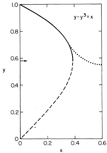
FIG. 3. Predicted dependence of y = (q_c/q_0)^2 on x = C_3(n/q_0)^2 , where q_0 is the wave vector at the transition [see Eq. (6)]. The dashed curve indicates that this region is physically inaccessible. The dotted curve shows the experimental results for \text{HoMo}_6\text{Se}_8 .
