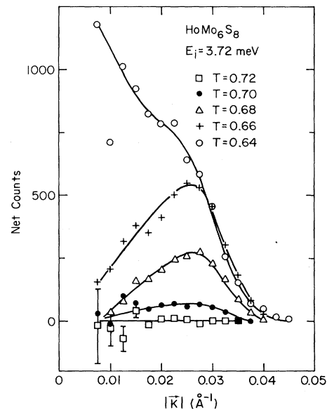
FIG. 1. Net scattering intensity, after subtraction of background at 2.0 K, as a function of wave vector for various temperatures. The peak at finite wave vector, which is limited in width by the instrumental resolution, indicates that an oscillatory magnetic state has developed on cooling.
