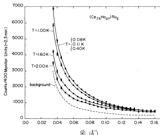
FIG. 7. Wave-vector dependence of the scattering at several temperatures. The solid curves are the result of a least-squares fit to the data assuming an Ornstein-Zernike correlation function.
