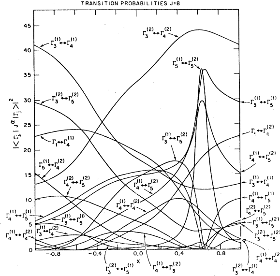
FIG. 3. Matrix elements |\langle \Gamma_i | J_z | \Gamma_j \rangle|^2 governing the crystal-field transition probabilities for neutron scattering as a function of the crystal-field parameter x (from Birgeneau, Ref. 23).
