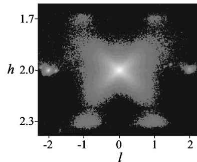
FIG. 1. Diffuse x-ray scattering data in the k_0 = 0.005 plane of reciprocal space simultaneously reveals polaron correlations, Huang scattering, and thermal diffuse scattering near the (200) Bragg reflection. The intensity scale of this CCD image is logarithmic, such that the strongest features are approximately 250 times more intense than the weakest features.
