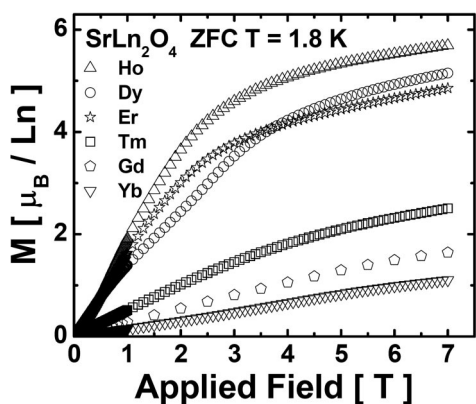
FIG. 12. The magnetization for \text{SrLn}_2\text{O}_4 materials as a function of applied field at 1.8 K. Zero-field cooling.
