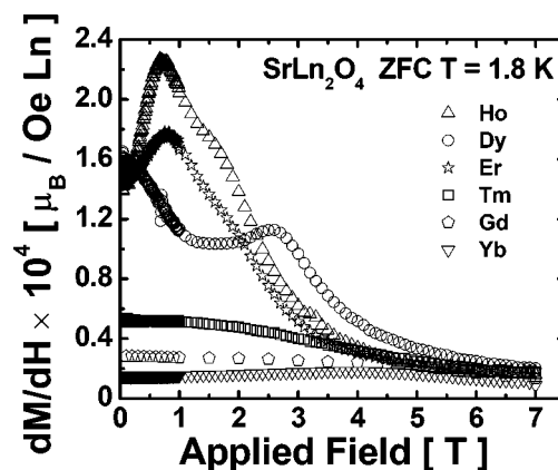
FIG. 13. The derivatives, dM/dH of the magnetization data in Fig. 12, as a function of applied field.
