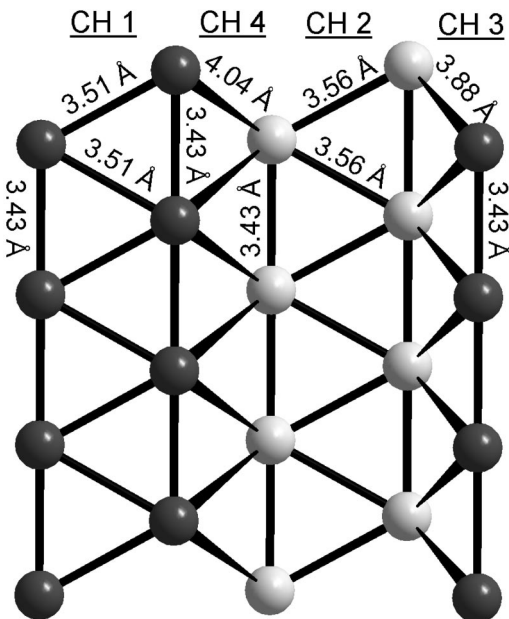
FIG. 5. Side view of the lanthanide chains, running parallel to the crystallographic c axis. L(1) shown as dark circles, L(2) shown as lighter circles. Lines connect lanthanide near neighbors. Interlanthanide distances are shown for the case of Dy. The primary chains, CH1 and CH2, have shorter L - L separations, and the secondary, or connecting chains, CH3 and CH4, have longer L - L distances. The shorter L - L distances along the spines of the chains are also seen.
