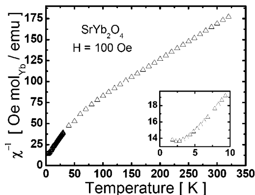
FIG. 11. The temperature dependence of the inverse magnetic susceptibility for \text{SrYb}_2\text{O}_4 between 320 and 2 K. Data taken on cooling in an applied field of 100 Oe. Inset: detail of the inverse susceptibility in the low-temperature region.
