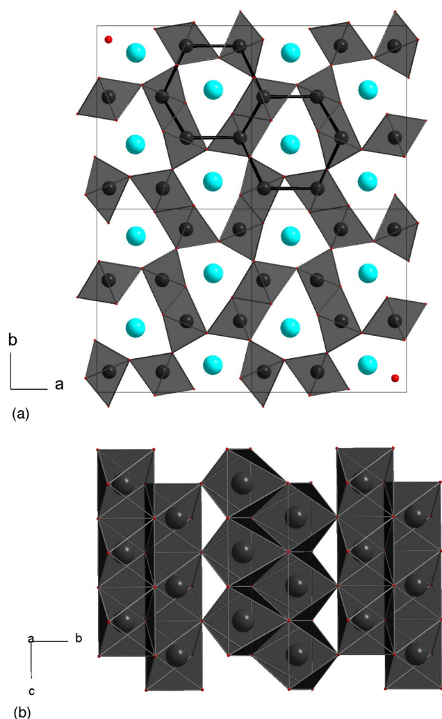
FIG. 2. (Color online) (a) The crystal structure of \text{SrDy}_2\text{O}_4 shown as an arrangement of \text{LO}_6 octahedra and isolated Sr atoms in channels, viewed down the crystallographic c axis. (b) The arrangement of \text{LO}_6 octahedra perpendicular to c showing both the double-row columns of octahedra, and the manner in which those columns share corner oxygens with each other.
