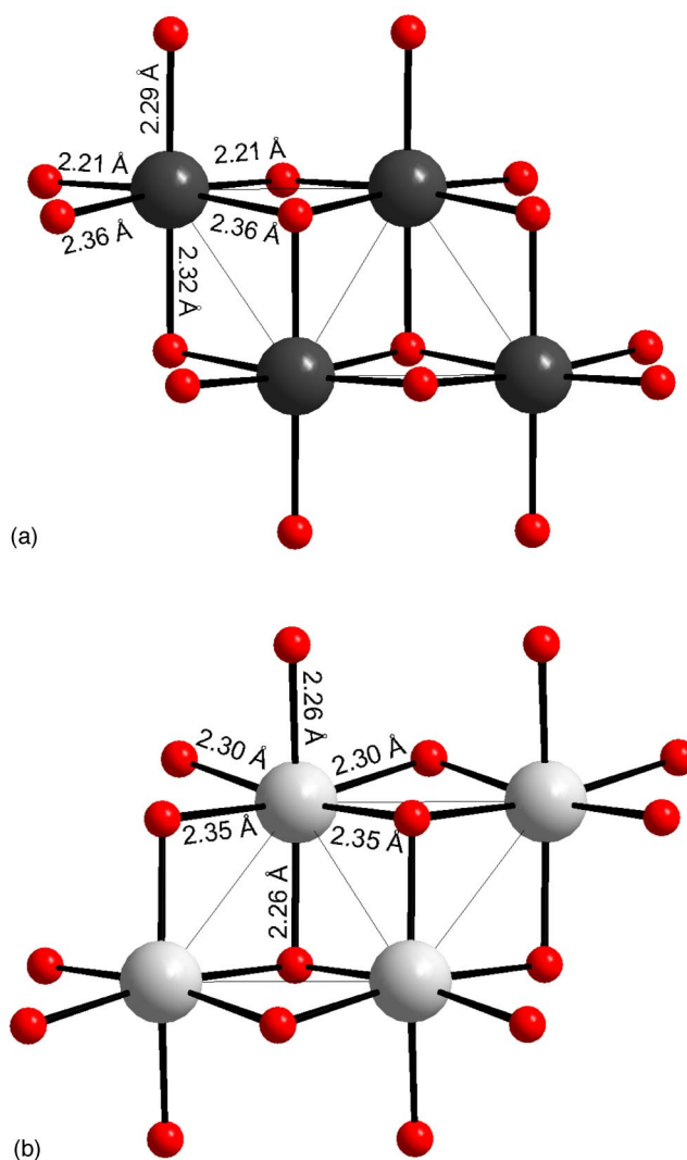
FIG. 3. (Color online) The geometries of the \text{LO}_6 octahedra in the double-row columns, for (a) L(1) , and (b) L(2) . The lanthanide-oxygen distances are shown for the case of \text{SrDy}_2\text{O}_4 . L(1) shown as larger dark circles, L(2) shown as larger lighter circles, oxygen as small black circles.
