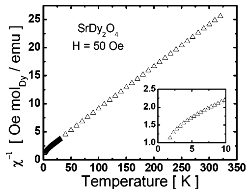
FIG. 7. The temperature dependence of the inverse magnetic susceptibility for \text{SrDy}_2\text{O}_4 between 320 and 2 K. Data taken on cooling in an applied field of 50 Oe. Inset: detail of the inverse susceptibility in the low-temperature region.
