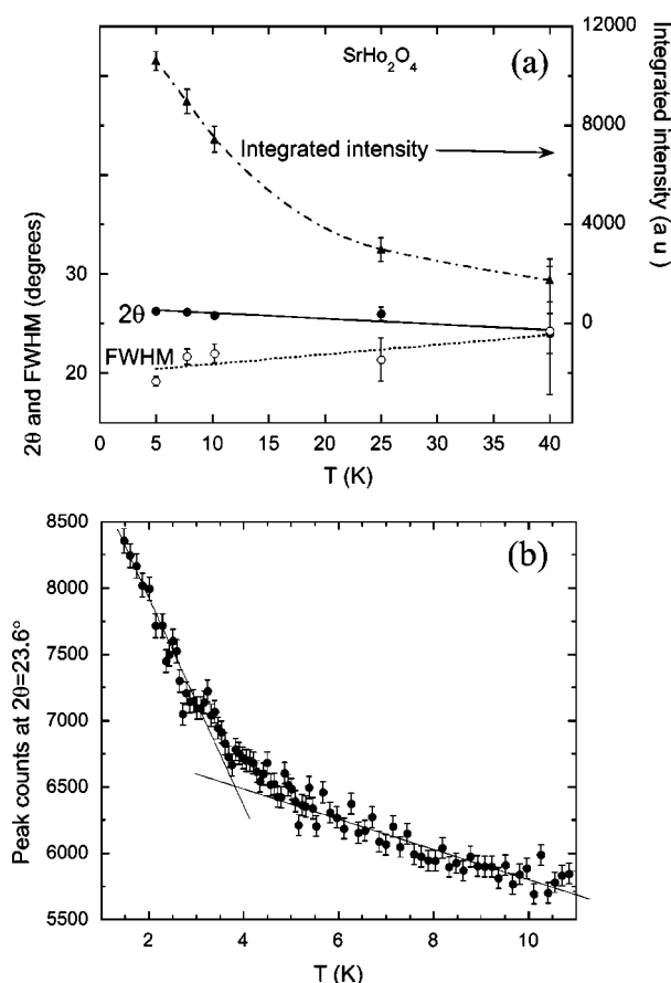
FIG. 17. (a) Plots of the integrated intensity, position, and FWHM as a function of temperature for the short-range order correlations in \text{SrHo}_2\text{O}_4 . (b) Intensity vs temperature at the 2D (02) peak position. The change in slope around 4 K indicates a crossover from short-range magnetic correlations to 2D long-range order.
