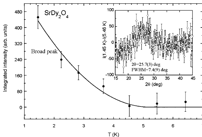
FIG. 14. A broad magnetic peak is observed below \sim 5 K in \text{SrDy}_2\text{O}_4 (inset), indicating that short-range magnetic order develops at low temperatures in this system.
