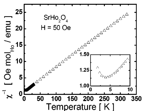
FIG. 8. The temperature dependence of the inverse magnetic susceptibility for \text{SrHo}_2\text{O}_4 between 320 and 2 K. Data taken on cooling in an applied field of 50 Oe. Inset: detail of the inverse susceptibility in the low-temperature region.
