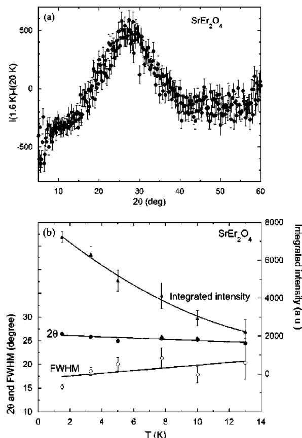
FIG. 15. (a) A very broad peak showing the short-range magnetic order develops below \sim 20 K in \text{SrEr}_2\text{O}_4 ; (b) integrated intensity, full width at half maximum (FWHM), and position of the broad peak as a function of temperature.
