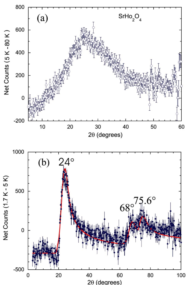
FIG. 16. (Color online) (a) Broad distribution of magnetic scattering at intermediate temperatures, indicating the development of short-range correlations in \text{SrHo}_2\text{O}_4 . This scattering begins to develop below \sim 40 K. (b) The magnetic scattering at low temperatures, indicating the development of two-dimensional long-range magnetic order. The solid curve is a fit assuming long-range order within the ab plane, and no correlations between planes.
