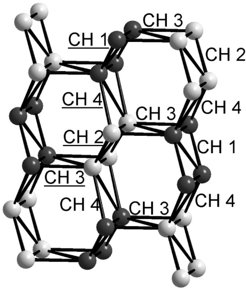
FIG. 4. Detailed view of the magnetic atom sublattice in the “honeycomb” direction in \text{SrDy}_2\text{O}_4 , showing the four lanthanide chains running perpendicular to the honeycomb net. Lines connect near neighbor lanthanides. L(1) shown as dark circles, L(2) shown as lighter circles.
