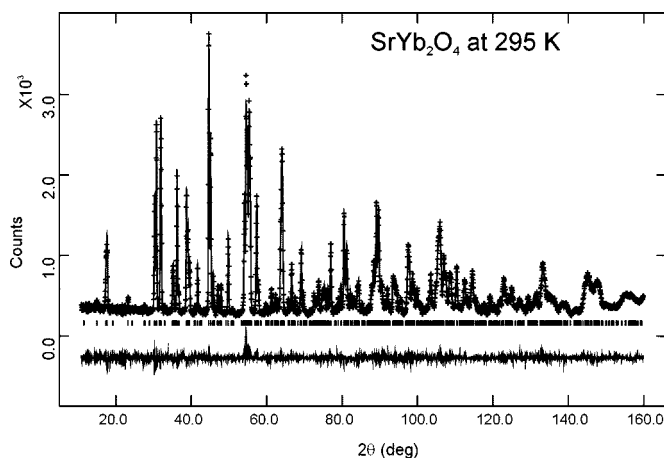
FIG. 1. Neutron powder-diffraction pattern of \text{SrYb}_2\text{O}_4 at ambient temperature. Upper curve: data and fit, short vertical lines, calculated peak positions. Lower curve: difference between observed and calculated pattern.
