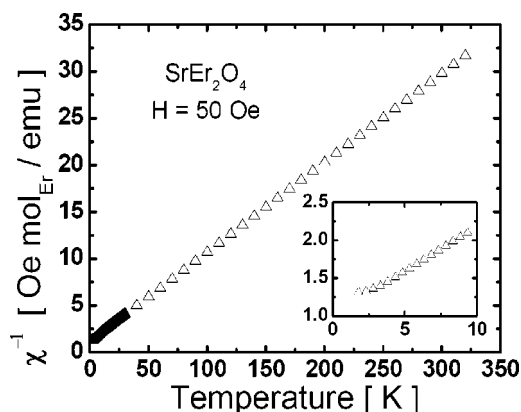
FIG. 9. The temperature dependence of the inverse magnetic susceptibility for \text{SrEr}_2\text{O}_4 between 320 and 2 K. Data taken on cooling in an applied field of 50 Oe. Inset: detail of the inverse susceptibility in the low-temperature region.
