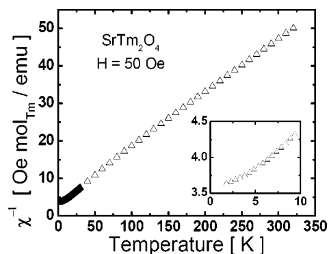
FIG. 10. The temperature dependence of the inverse magnetic susceptibility for \text{SrTm}_2\text{O}_4 between 320 and 2 K. Data taken on cooling in an applied field of 50 Oe. Inset: detail of the inverse susceptibility in the low-temperature region.
